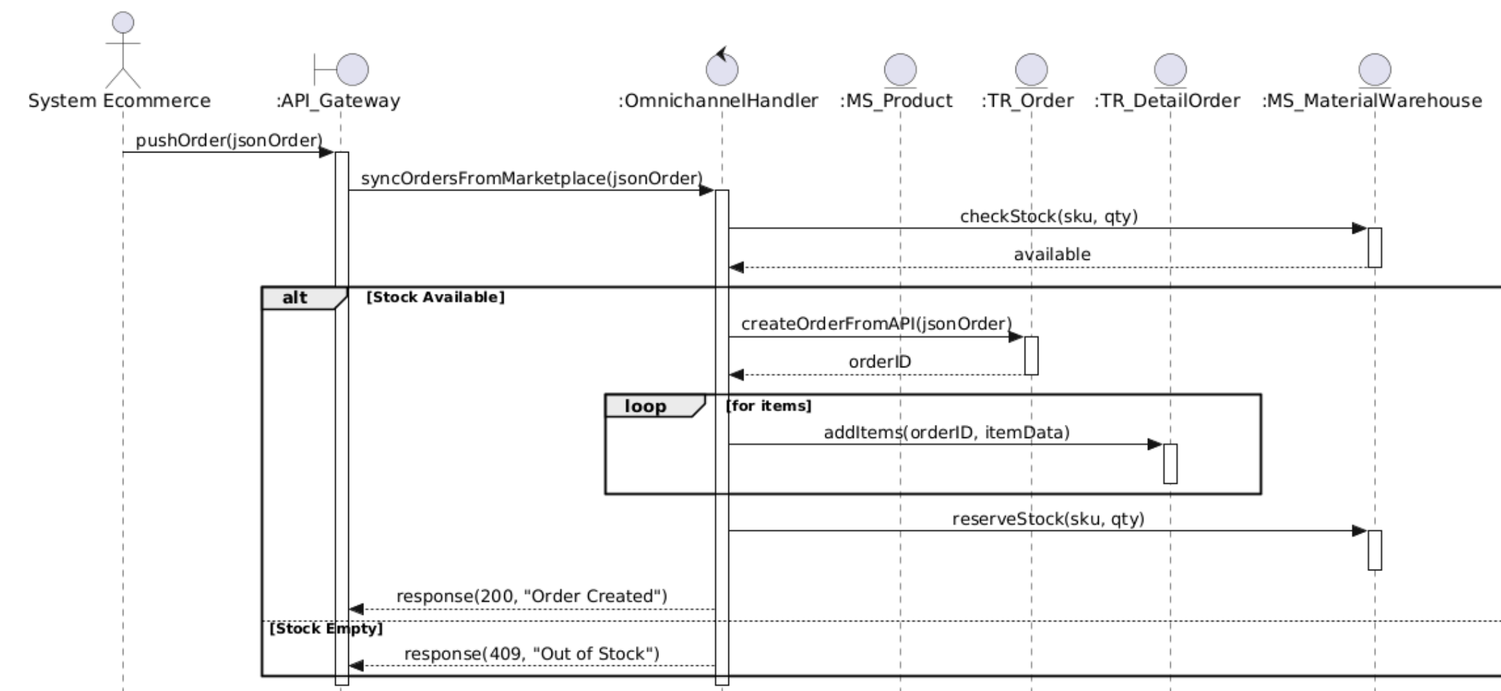
First Cut Sequence Diagram : Mengelola Pesanan (Omnichannel)
