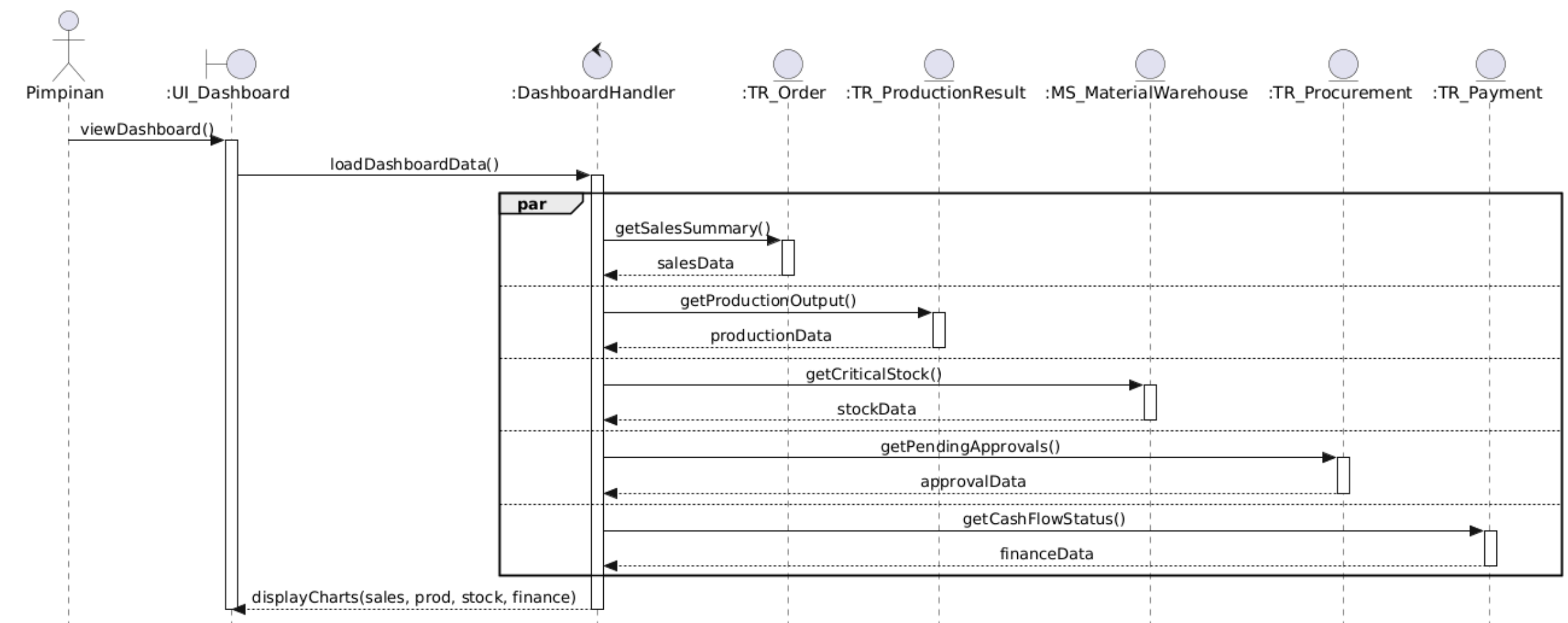
Sequence Diagram: Memantau Kinerja Bisnis (Dashboard)
