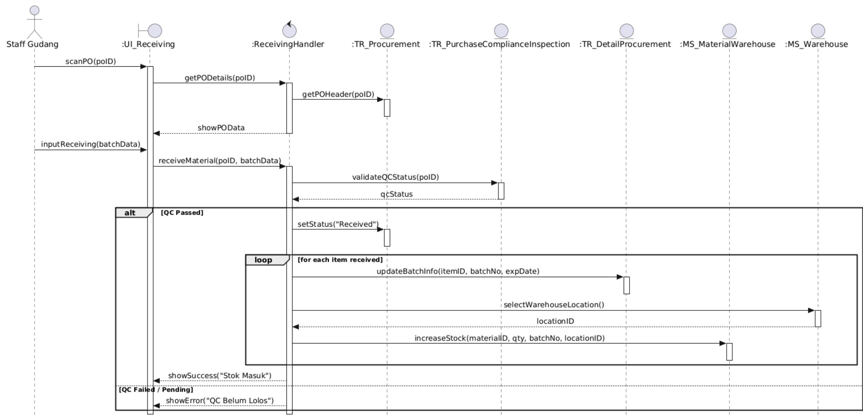
First Cut Sequece Diagram : Manage Penerimaan Bahan Baku
