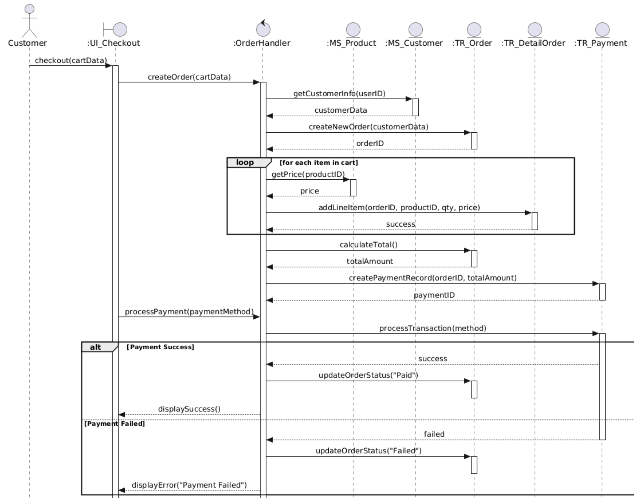
First Cut Sequence Diagram: Memesan Barang (B2C)
